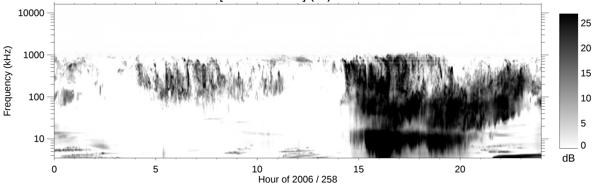
RPWS [ABCH1H2/Ex] (-B) 2006/09/15
