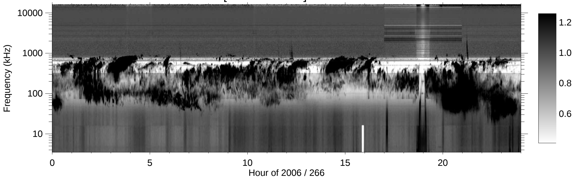
RPWS [ABCH1H2/Ex] (-B) 2006/09/23
