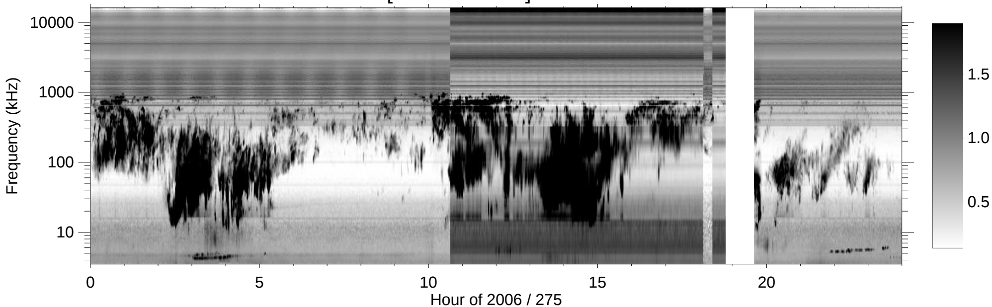
RPWS [ABCH1H2/Ex] (-B) 2006/10/02
