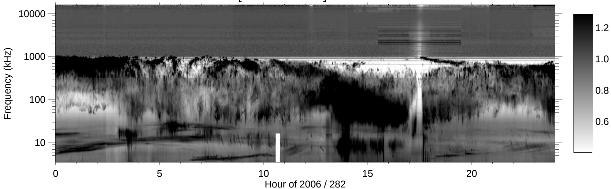
RPWS [ABCH1H2/Ex] (-B) 2006/10/09
