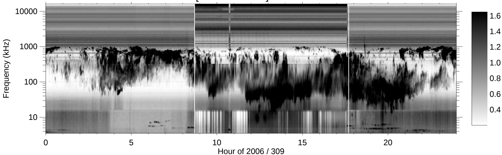
RPWS [ABCH1H2/Ex] (-B) 2006/11/05
