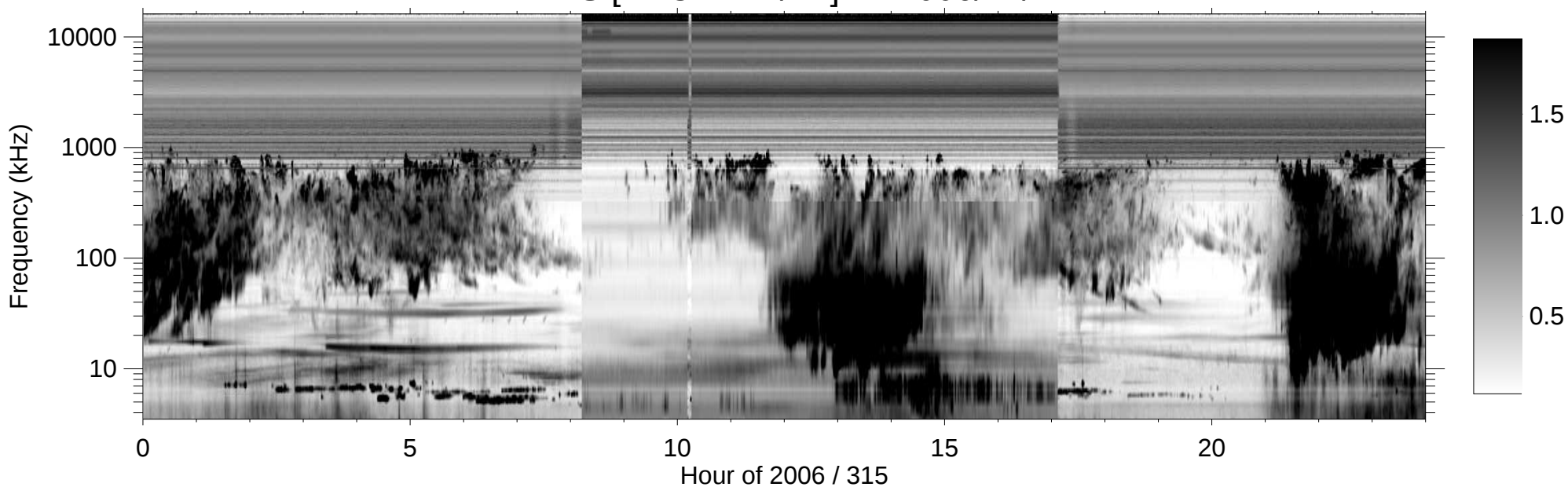
RPWS [ABCH1H2/Ex] (-B) 2006/11/11
