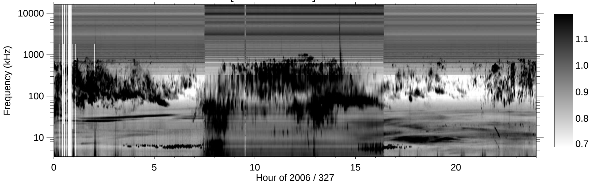
RPWS [ABCH1H2/Ex] (-B) 2006/11/23
