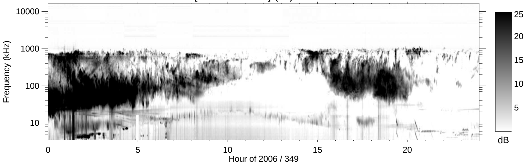
RPWS [ABCH1H2/Ex] (-B) 2006/12/15
