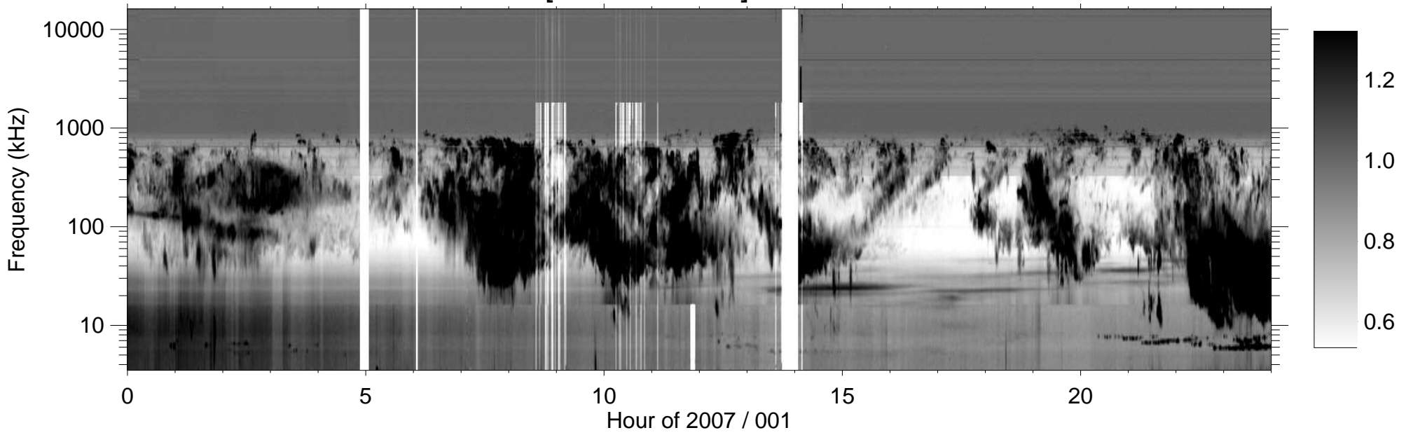
RPWS [ABCH1H2/Ex] (-B) 2007/01/01
