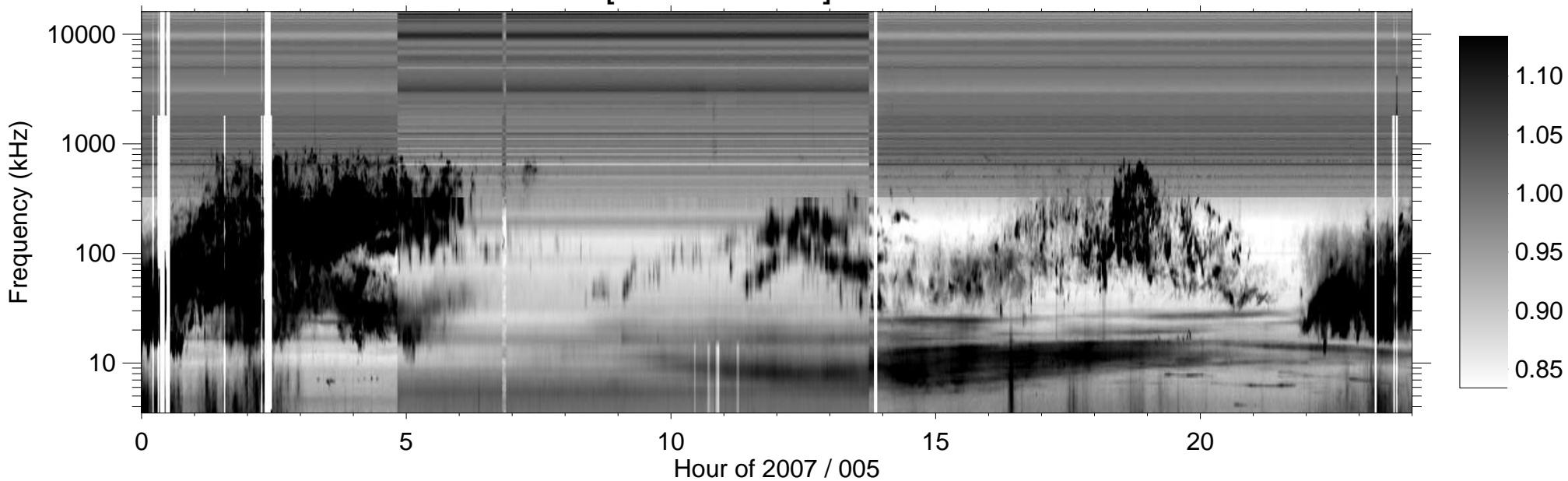
RPWS [ABCH1H2/Ex] (-B) 2007/01/05
