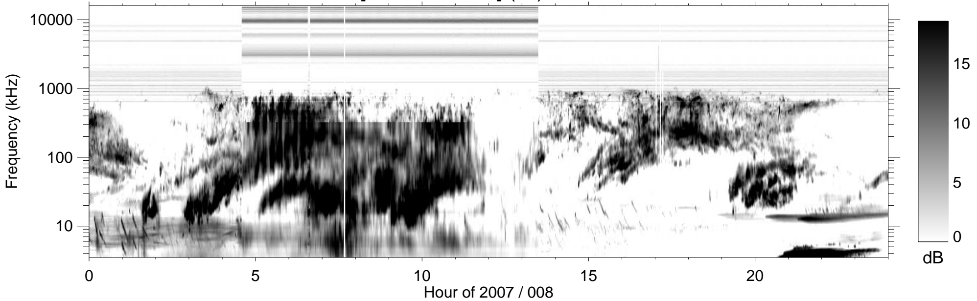
RPWS [ABCH1H2/Ex] (-B) 2007/01/08
