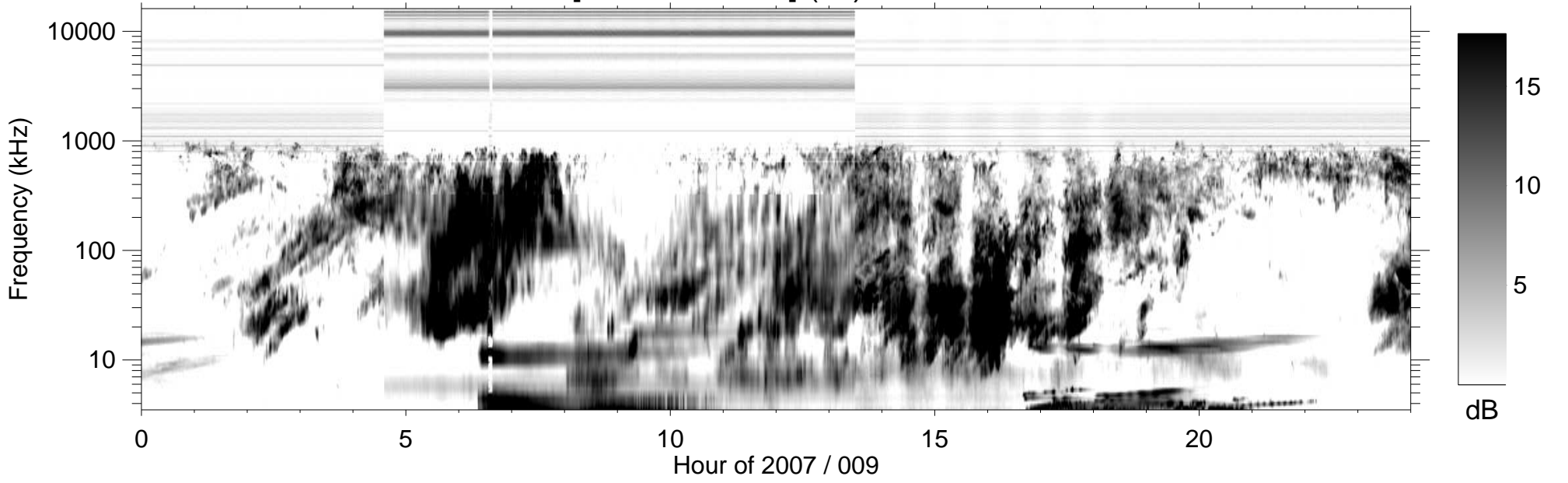
RPWS [ABCH1H2/Ex] (-B) 2007/01/09
