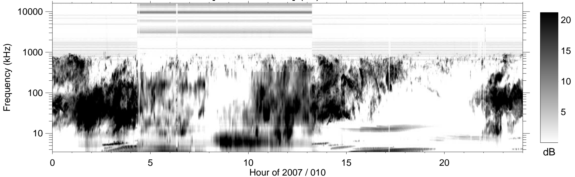
RPWS [ABCH1H2/Ex] (-B) 2007/01/10
