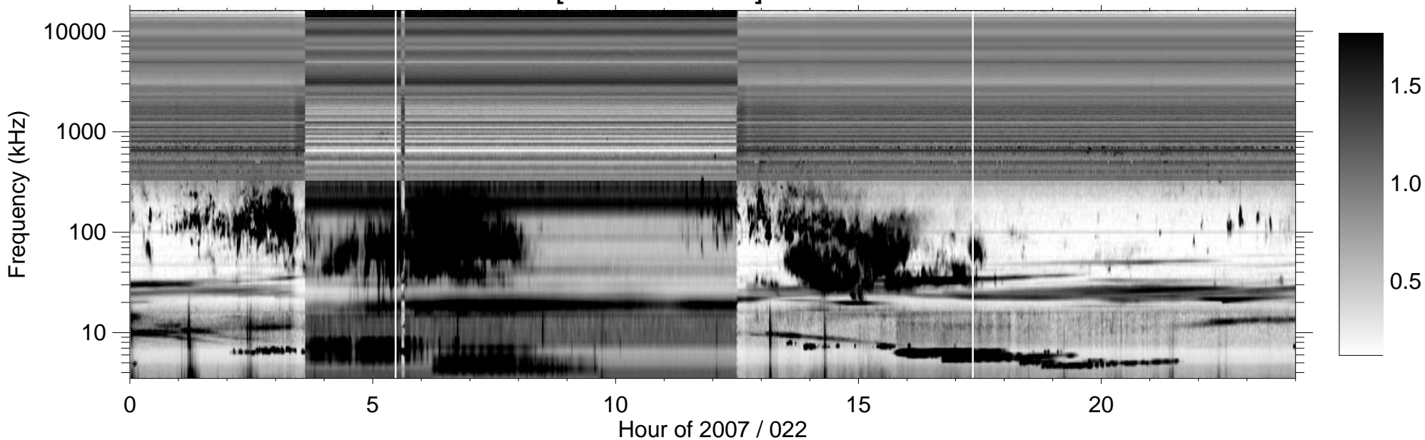
RPWS [ABCH1H2/Ex] (-B) 2007/01/22
