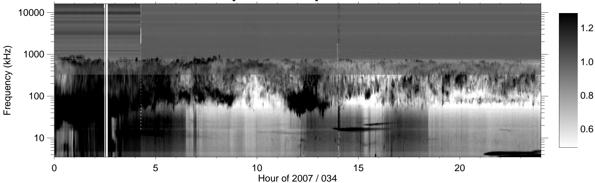
RPWS [ABCH1H2/Ex] (-B) 2007/02/03
