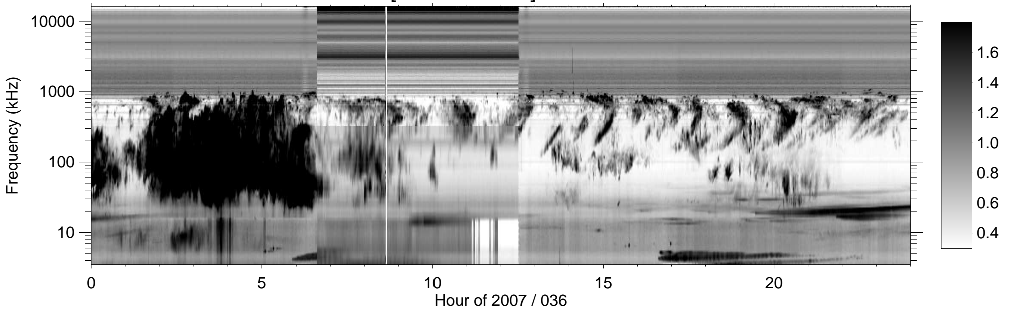
RPWS [ABCH1H2/Ex] (-B) 2007/02/05
