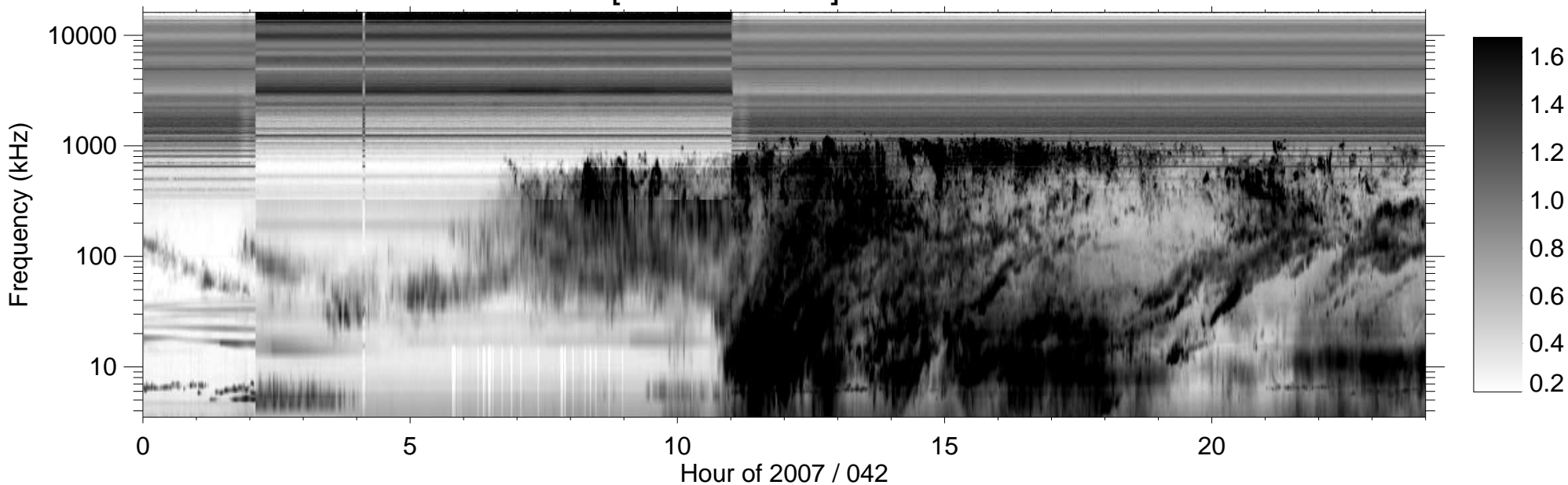
RPWS [ABCH1H2/Ex] (-B) 2007/02/11
