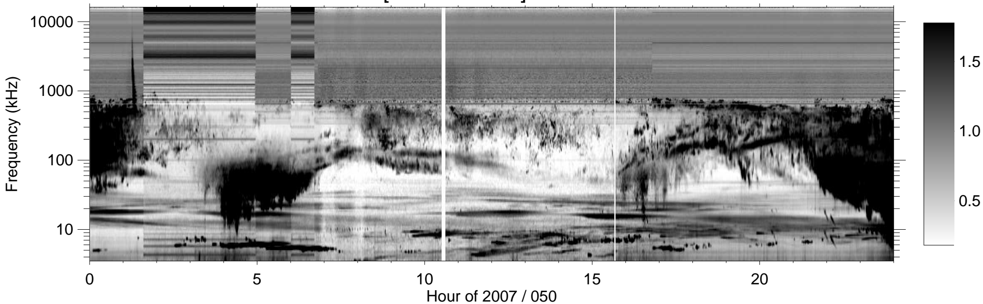
RPWS [ABCH1H2/Ex] (-B) 2007/02/19
