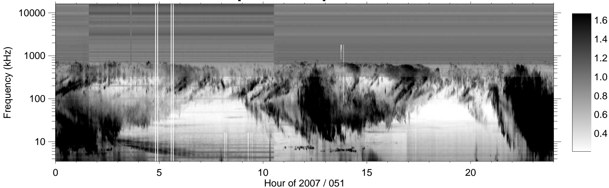
RPWS [ABCH1H2/Ex] (-B) 2007/02/20
