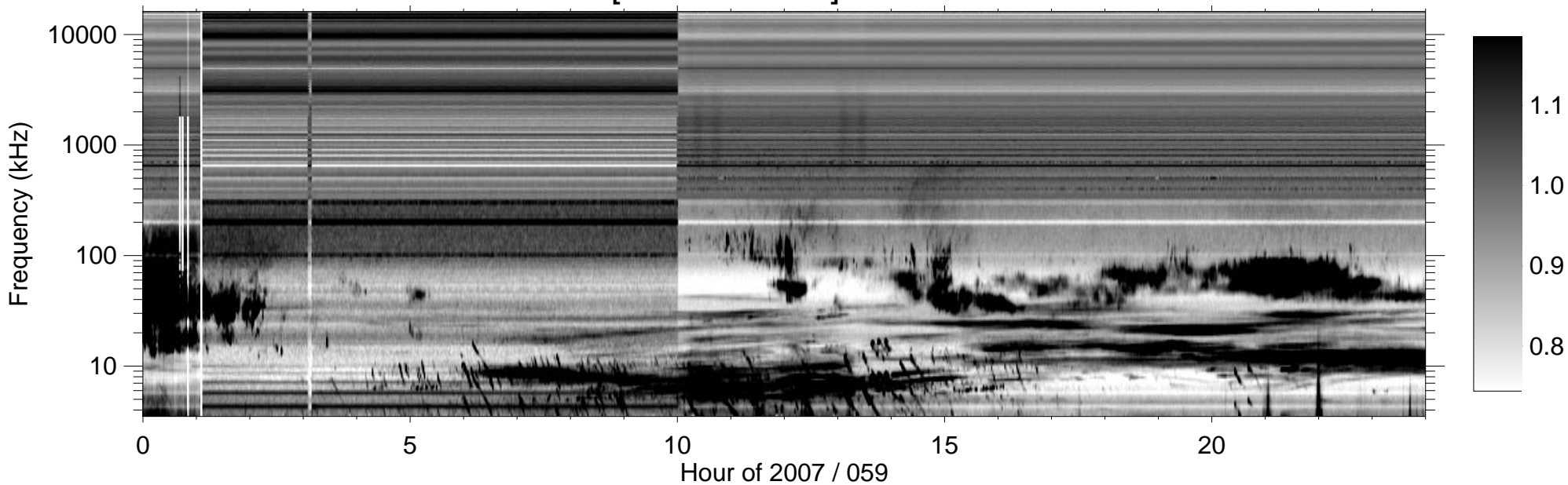
RPWS [ABCH1H2/Ex] (-B) 2007/02/28
