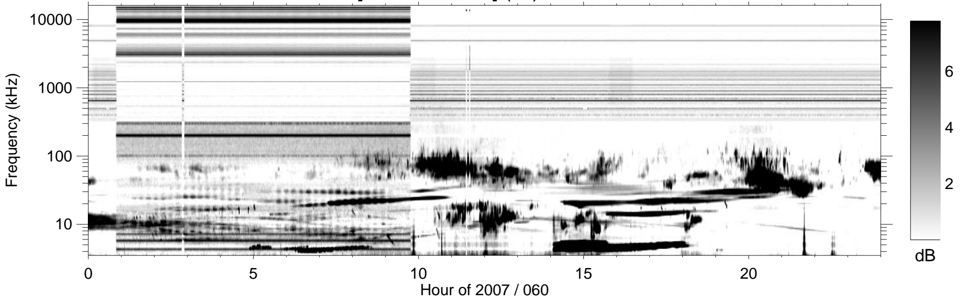
RPWS [ABCH1H2/Ex] (-B) 2007/03/01
