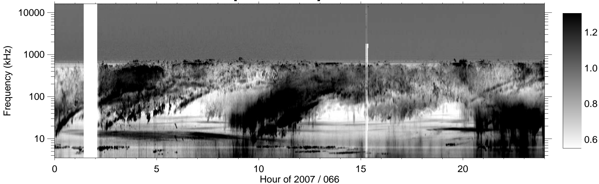
RPWS [ABCH1H2/Ex] (-B) 2007/03/07
