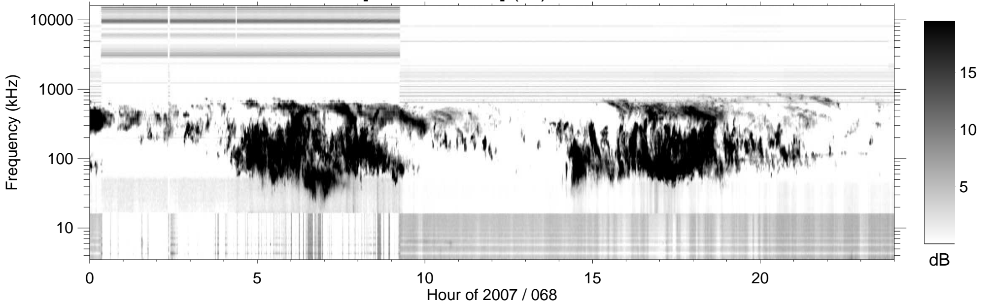
RPWS [ABCH1H2/Ex] (-B) 2007/03/09
