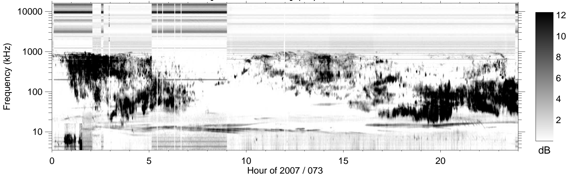
RPWS [ABCH1H2/Ex] (-B) 2007/03/14
