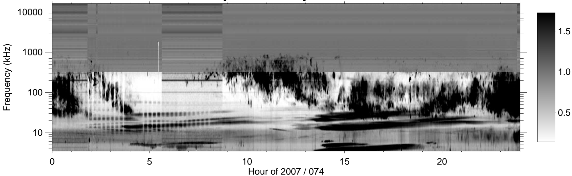
RPWS [ABCH1H2/Ex] (-B) 2007/03/15
