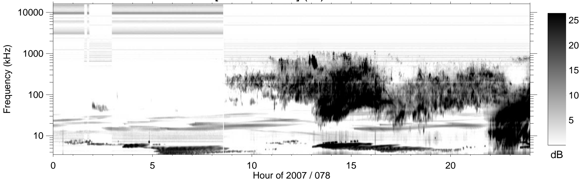
RPWS [ABCH1H2/Ex] (-B) 2007/03/19
