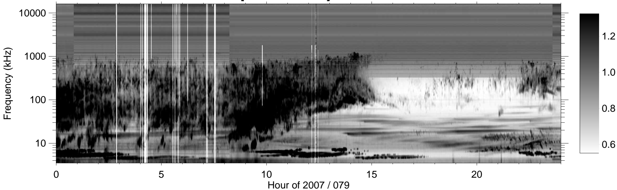
RPWS [ABCH1H2/Ex] (-B) 2007/03/20
