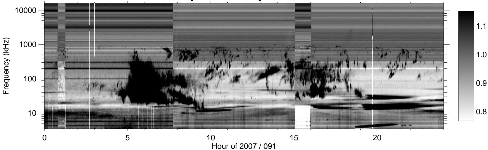
RPWS [ABCH1H2/Ex] (-B) 2007/04/01
