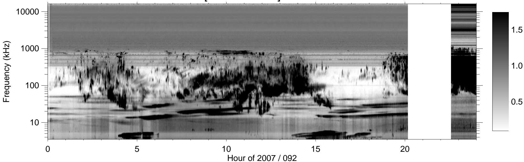
RPWS [ABCH1H2/Ex] (-B) 2007/04/02
