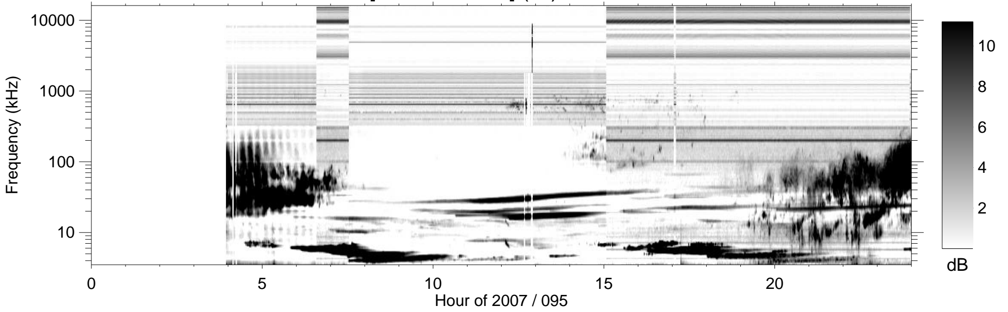
RPWS [ABCH1H2/Ex] (-B) 2007/04/05
