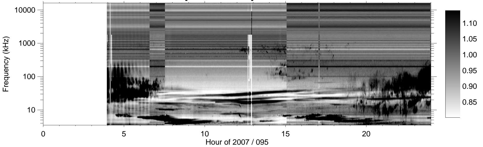
RPWS [ABCH1H2/Ex] (-B) 2007/04/05
