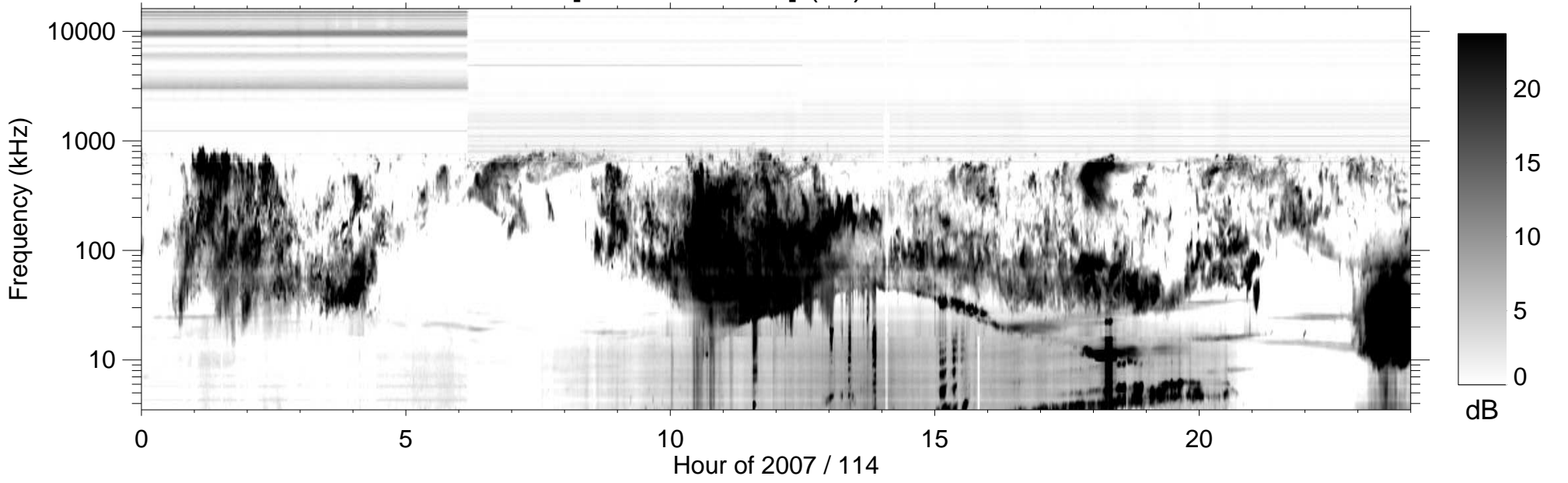
RPWS [ABCH1H2/Ex] (-B) 2007/04/24
