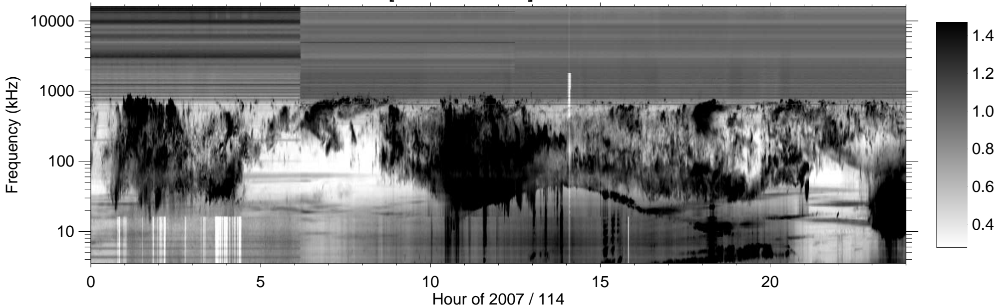
RPWS [ABCH1H2/Ex] (-B) 2007/04/24
