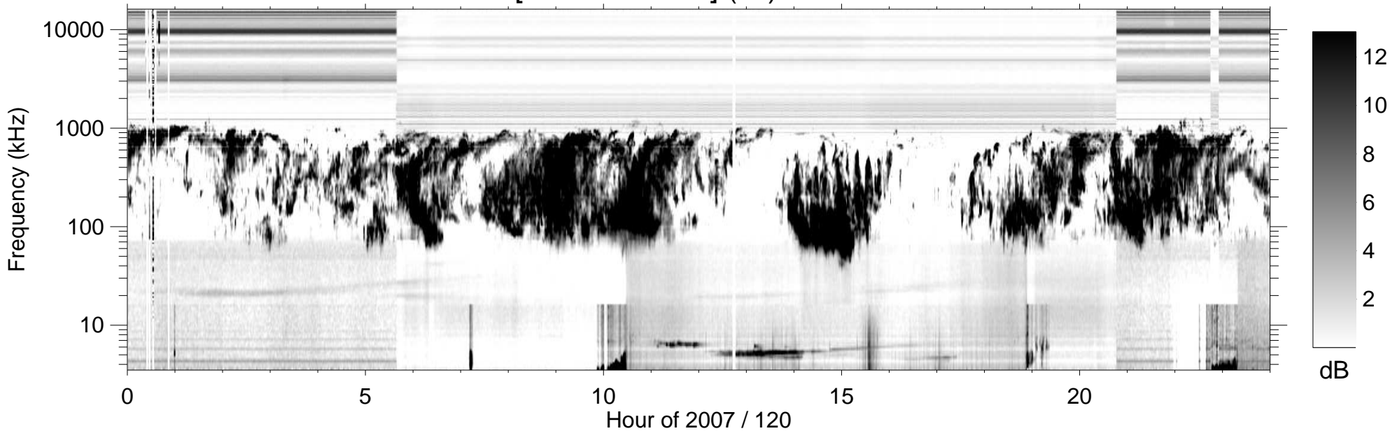
RPWS [ABCH1H2/Ex] (-B) 2007/04/30
