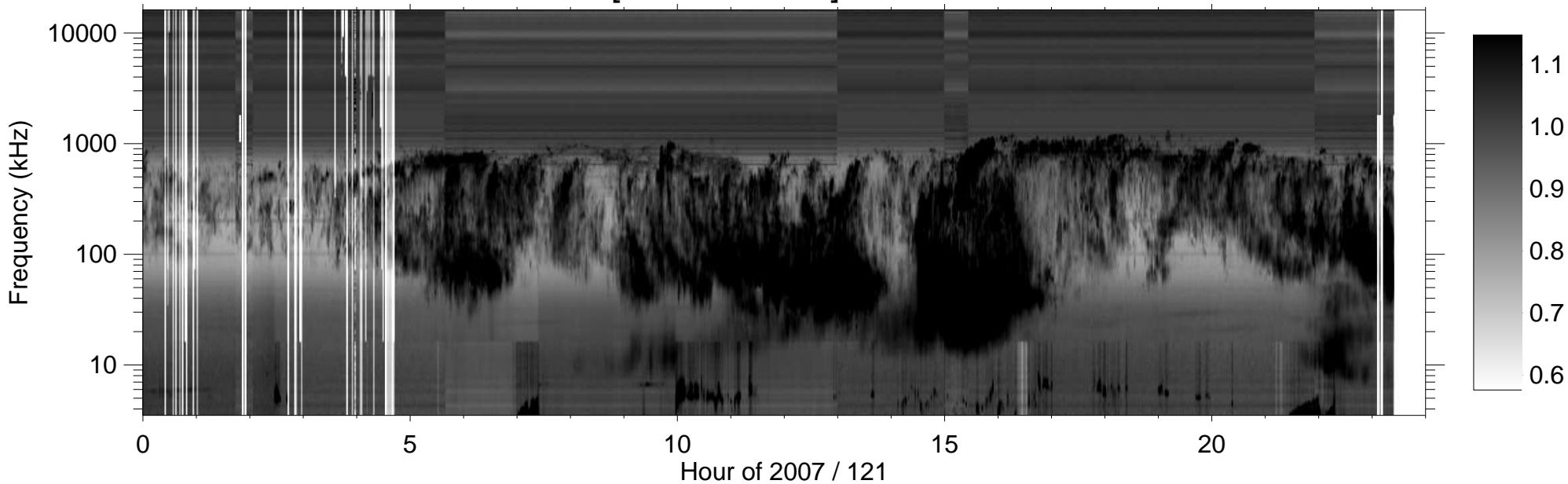
RPWS [ABCH1H2/Ex] (-B) 2007/05/01
