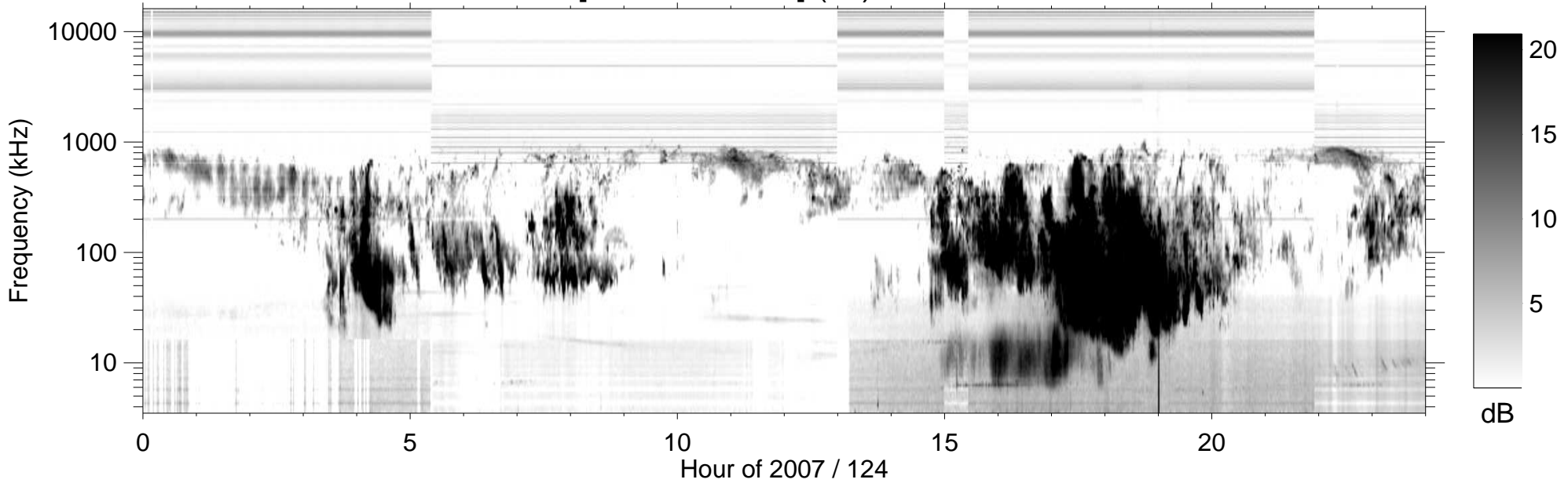
RPWS [ABCH1H2/Ex] (-B) 2007/05/04
