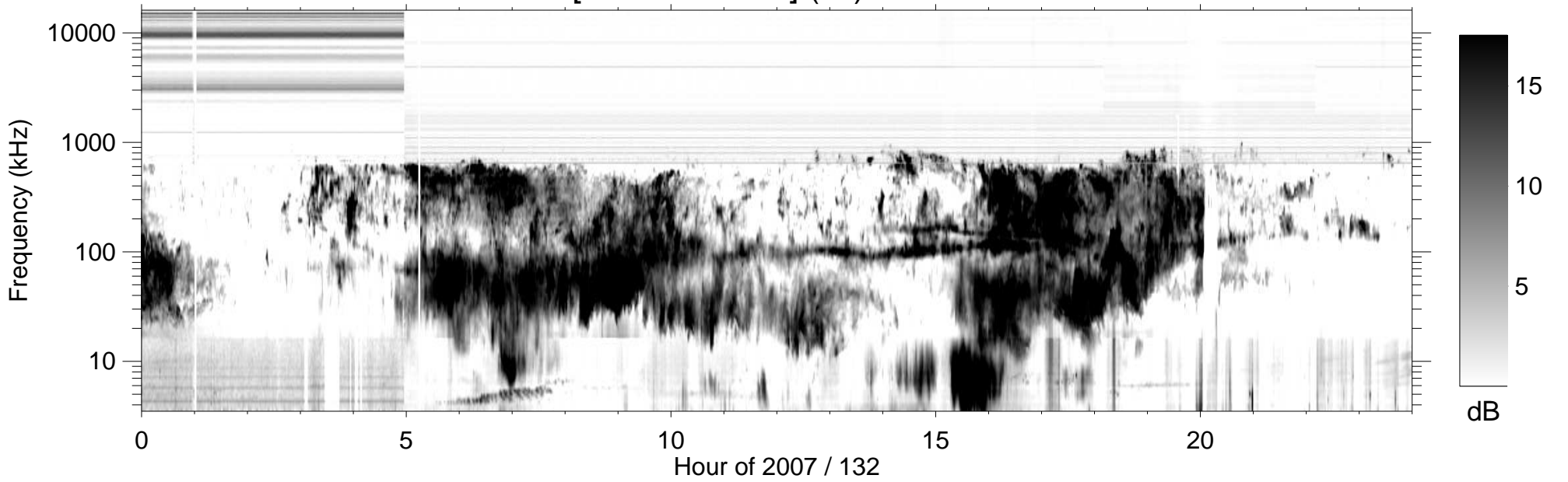
RPWS [ABCH1H2/Ex] (-B) 2007/05/12
