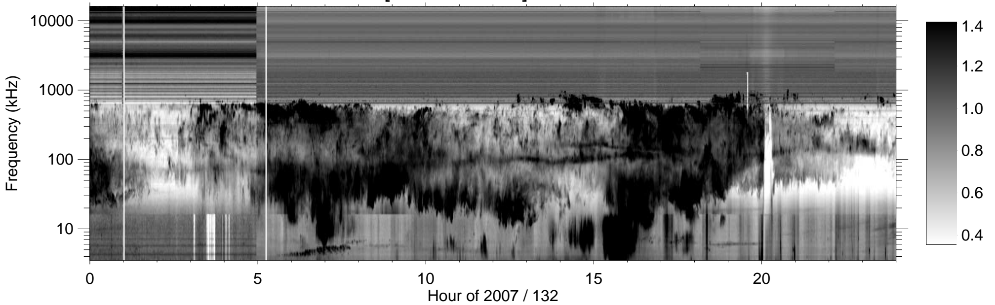
RPWS [ABCH1H2/Ex] (-B) 2007/05/12
