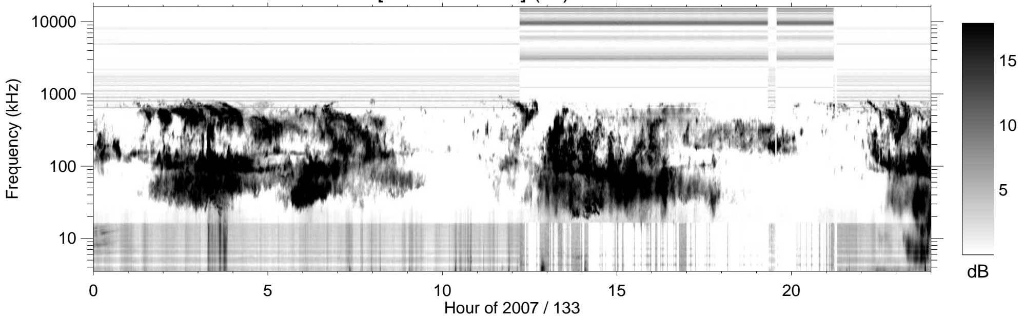
RPWS [ABCH1H2/Ex] (-B) 2007/05/13
