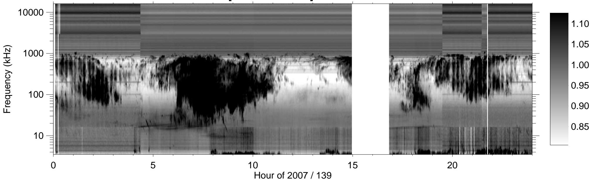
RPWS [ABCH1H2/Ex] (-B) 2007/05/19
