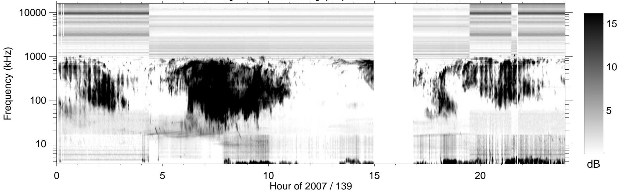
RPWS [ABCH1H2/Ex] (-B) 2007/05/19
