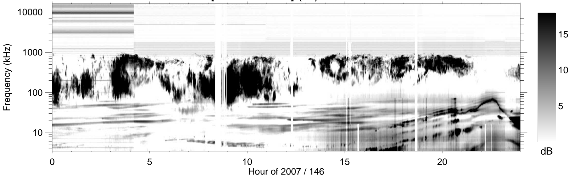
RPWS [ABCH1H2/Ex] (-B) 2007/05/26
