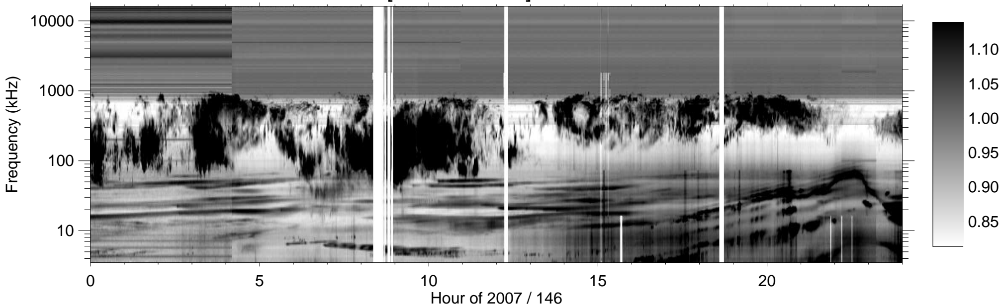
RPWS [ABCH1H2/Ex] (-B) 2007/05/26
