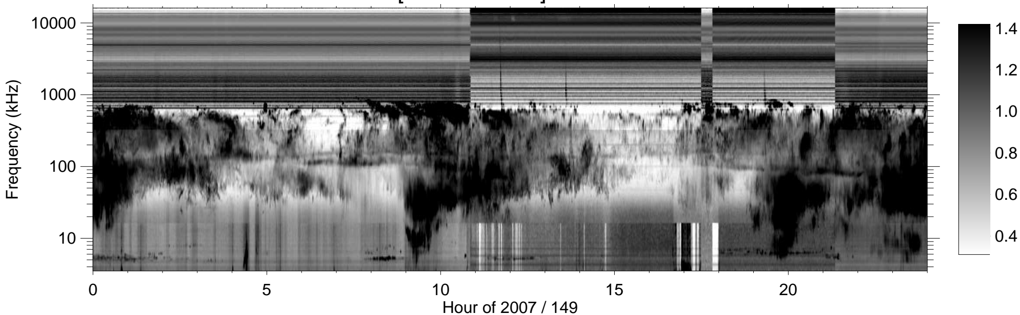
RPWS [ABCH1H2/Ex] (-B) 2007/05/29
