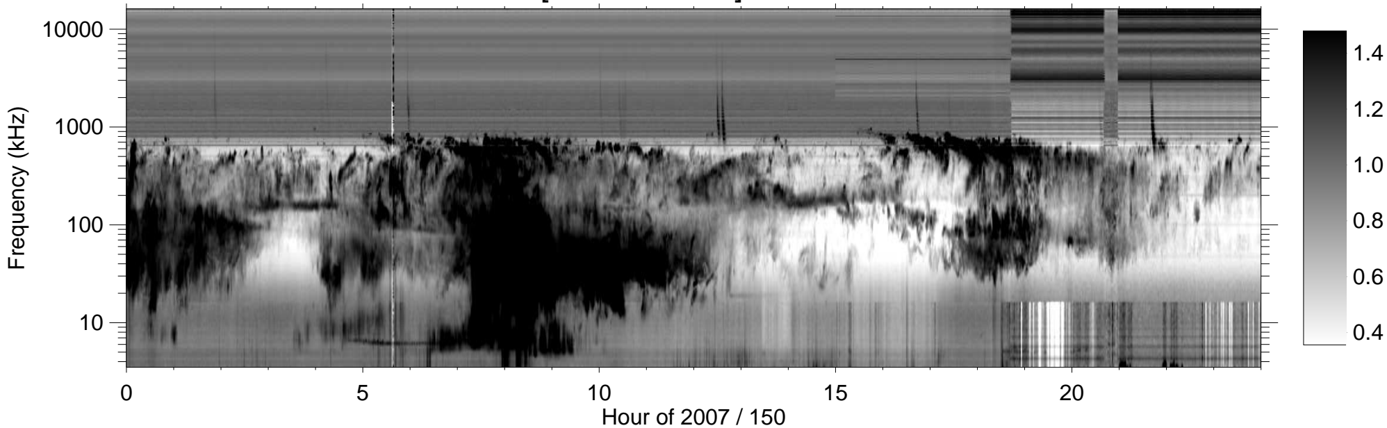
RPWS [ABCH1H2/Ex] (-B) 2007/05/30
