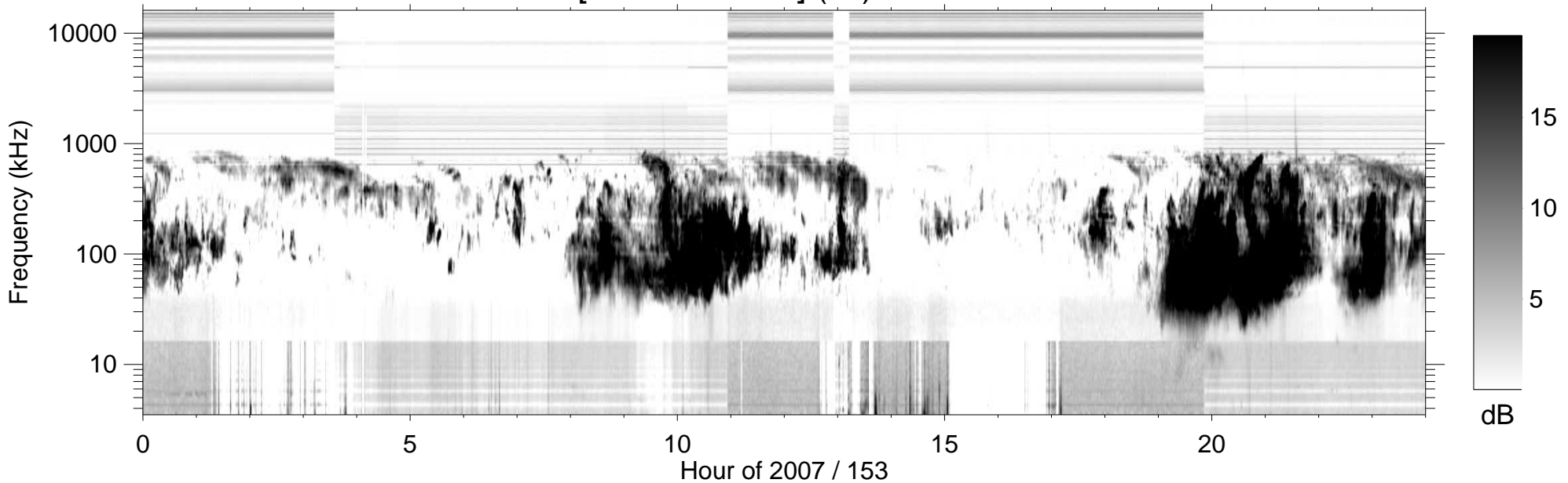
RPWS [ABCH1H2/Ex] (-B) 2007/06/02
