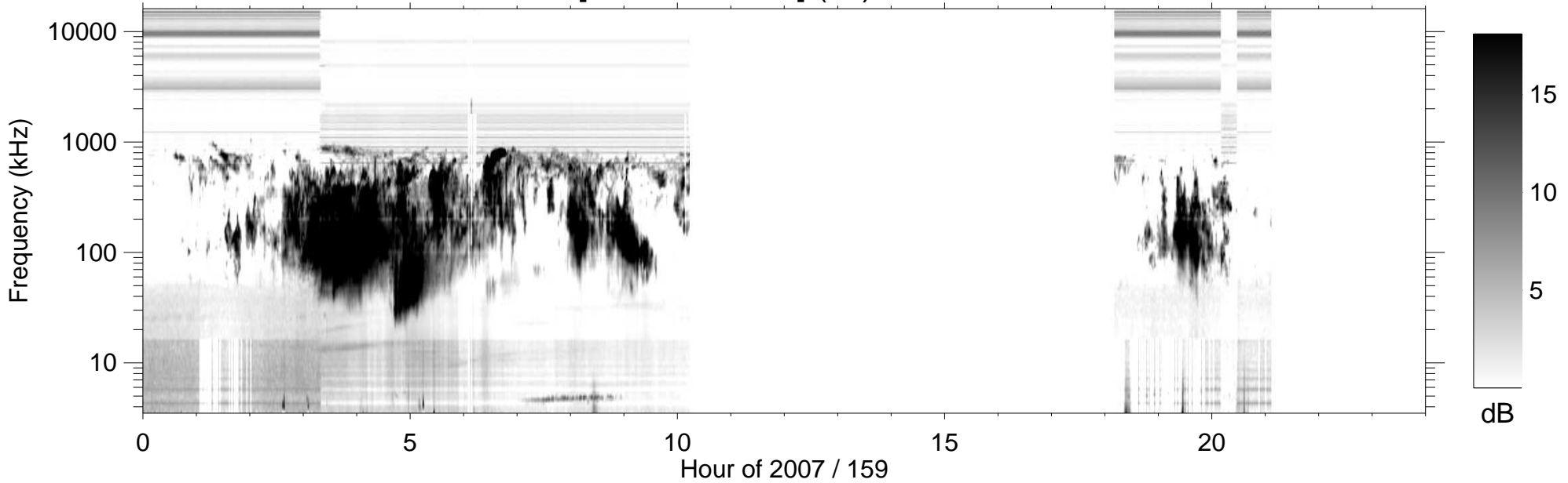
RPWS [ABCH1H2/Ex] (-B) 2007/06/08
