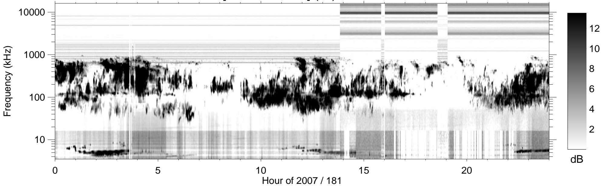
RPWS [ABCH1H2/Ex] (-B) 2007/06/30
