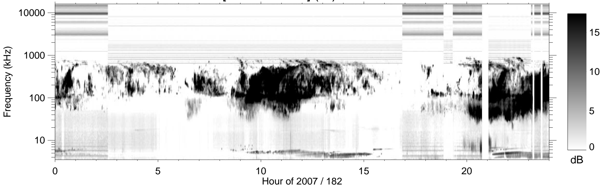
RPWS [ABCH1H2/Ex] (-B) 2007/07/01
