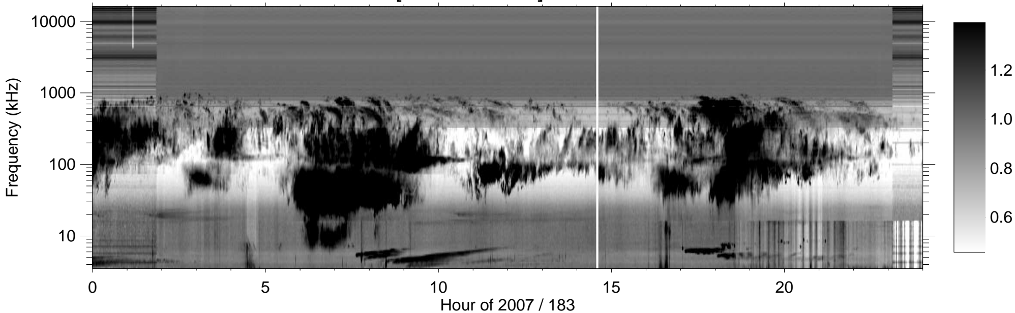
RPWS [ABCH1H2/Ex] (-B) 2007/07/02
