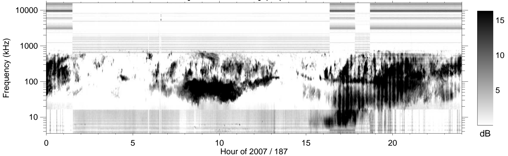
RPWS [ABCH1H2/Ex] (-B) 2007/07/06
