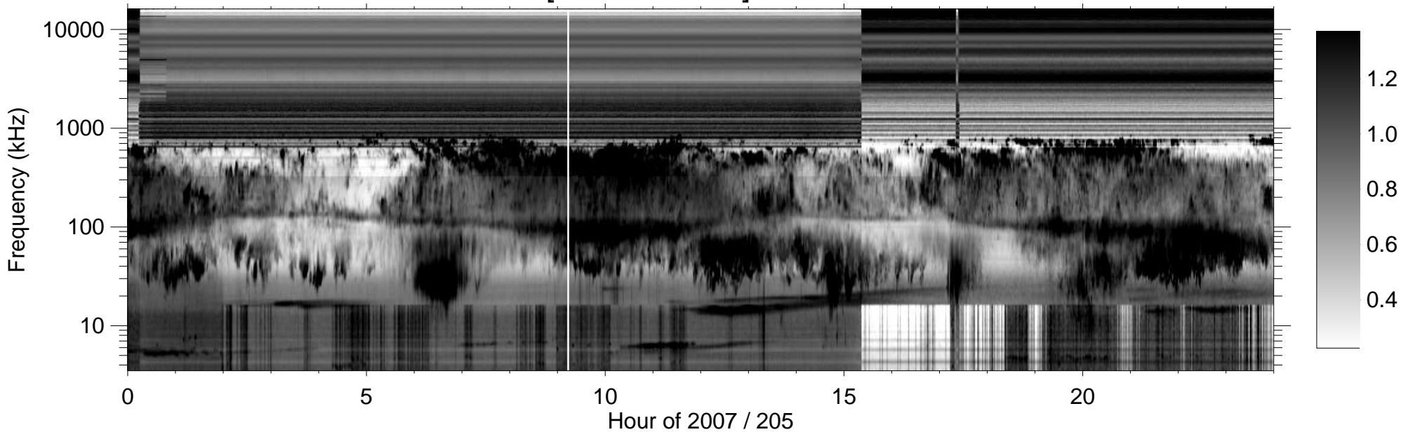
RPWS [ABCH1H2/Ex] (-B) 2007/07/24
