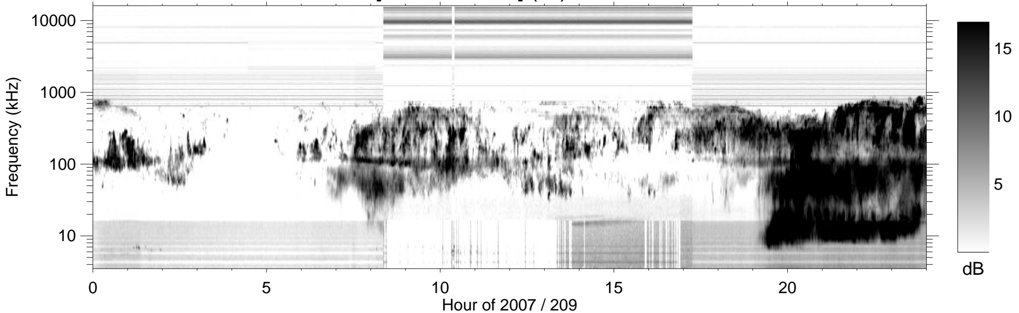
RPWS [ABCH1H2/Ex] (-B) 2007/07/28
