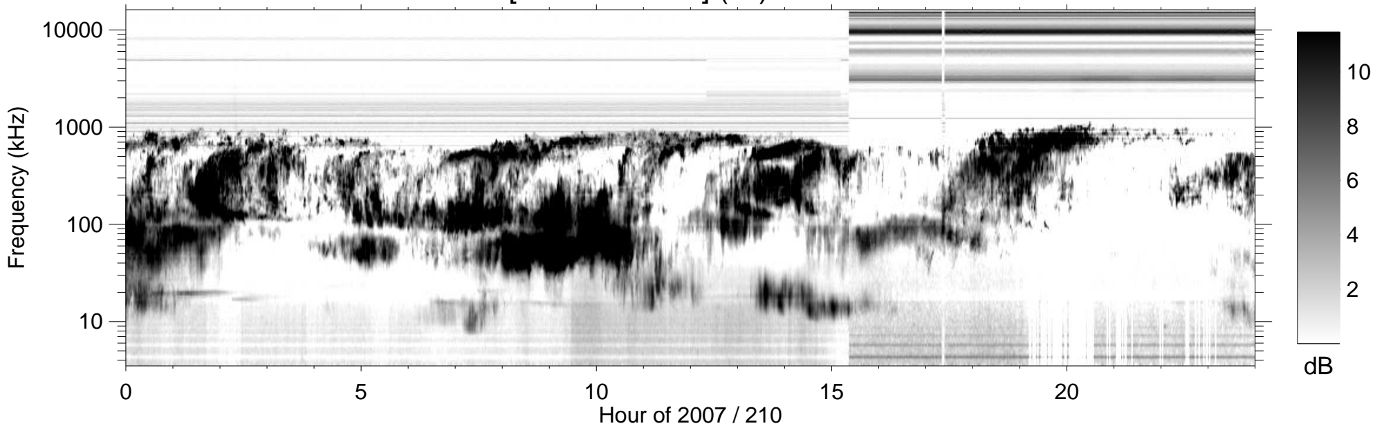
RPWS [ABCH1H2/Ex] (-B) 2007/07/29
