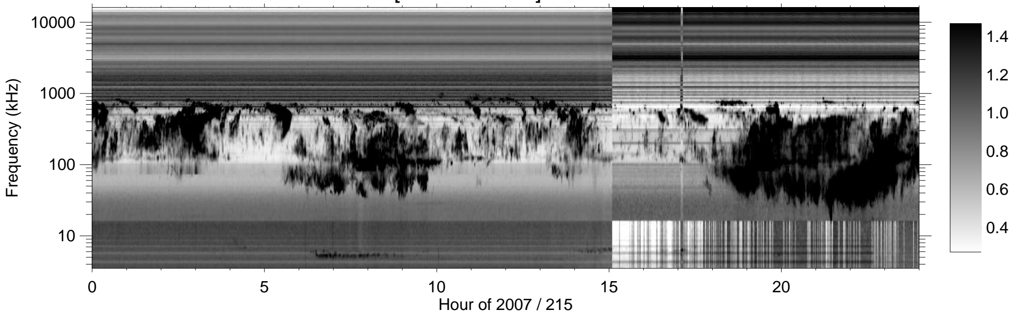
RPWS [ABCH1H2/Ex] (-B) 2007/08/03
